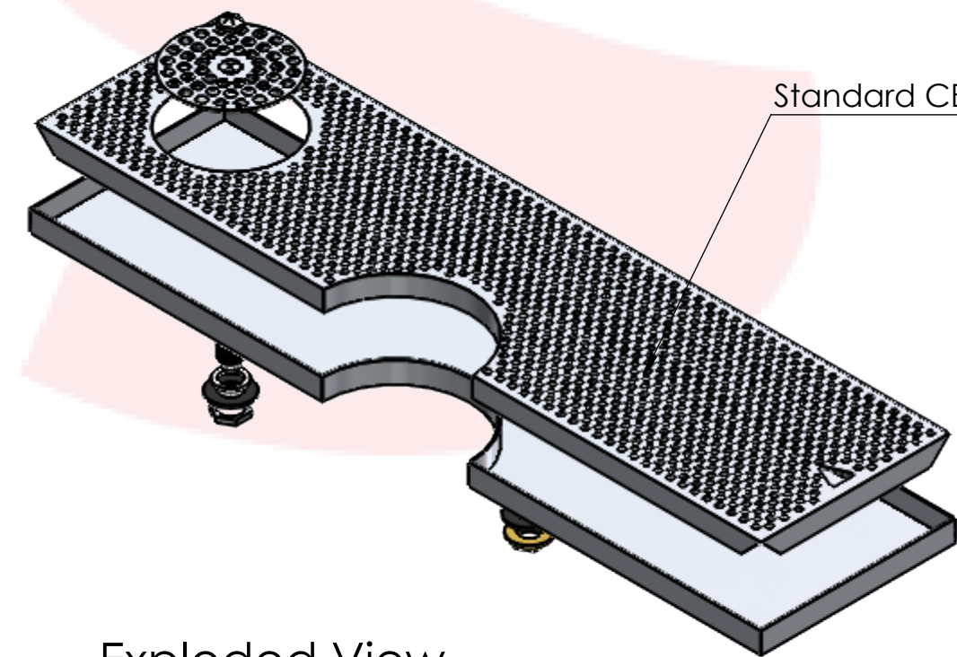
Exploded View
